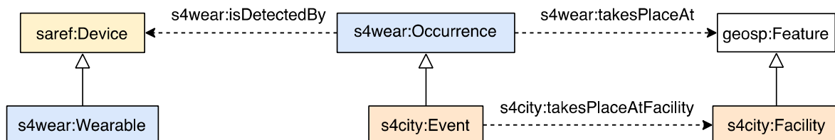
Figure 6: Occurrence model
