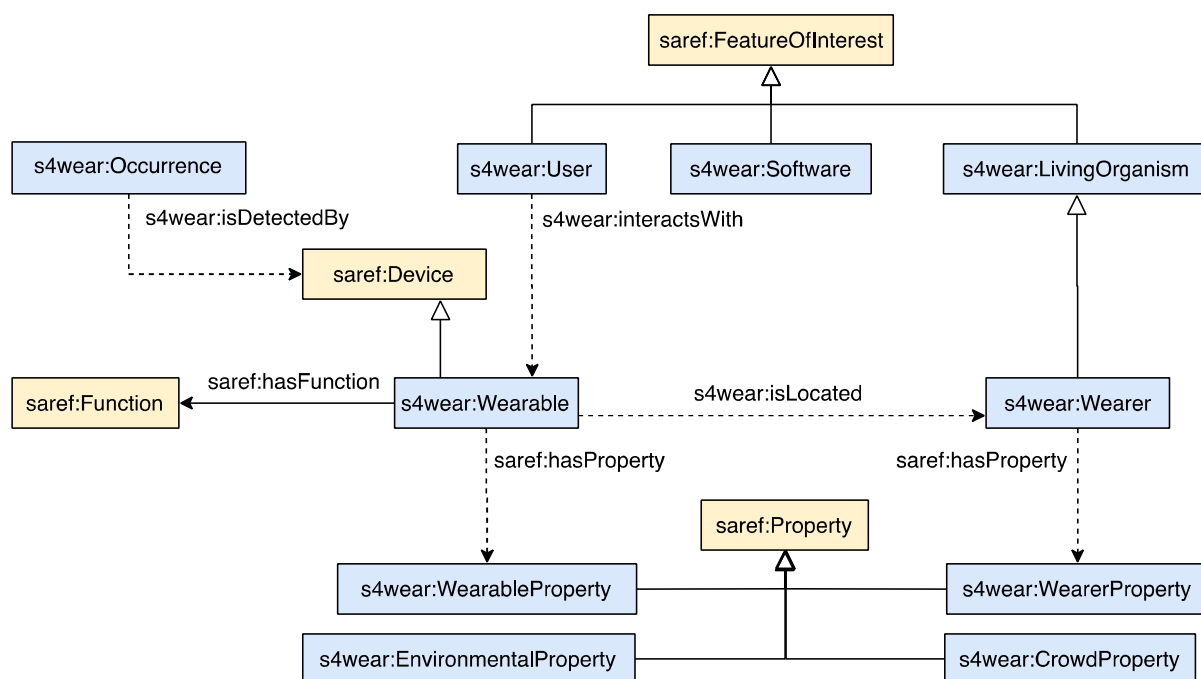
Figure 1: SAREF4WEAR overview
