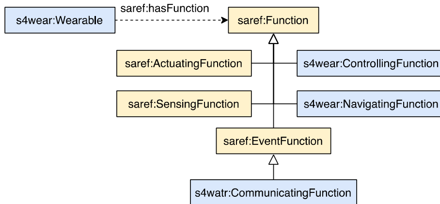
Figure 5: Function model
