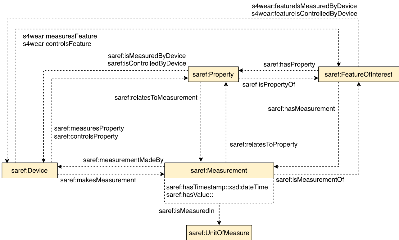
Figure 2: Measurement model
