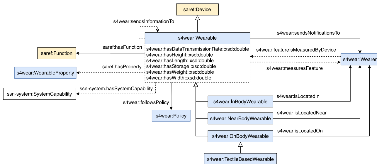
Figure 4: Wearable model
